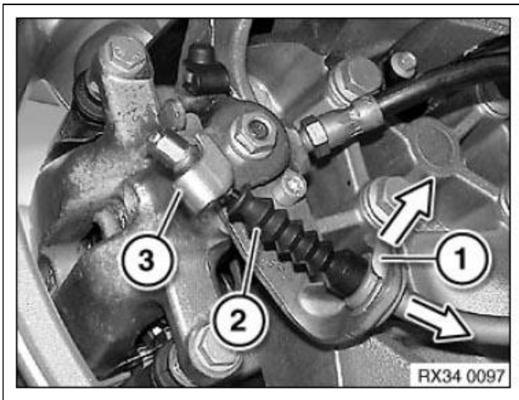
Fig 5: Removing Locking Clip
