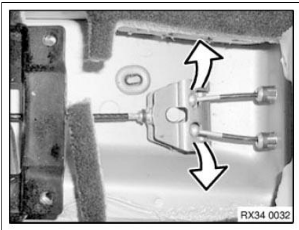
Fig 2: Removing Parking Brake Bowden Cables From Balance Arm
