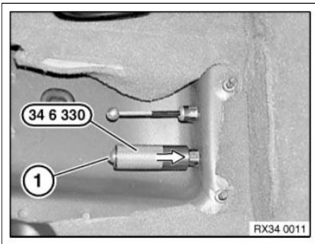
Fig 3: Sliding Special Tool (34 6 330) Onto Barbs Of Parking Brake Bowden Cable
