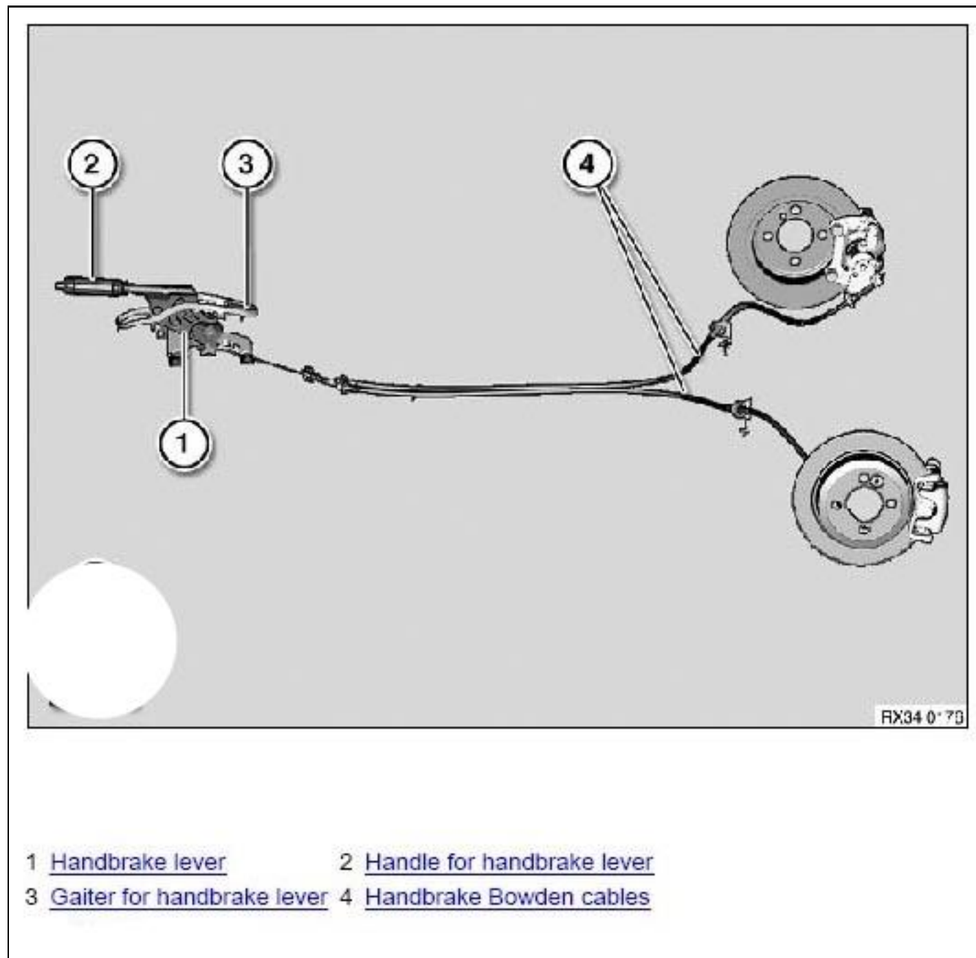
Fig 1: Overview Of Parking Brake
