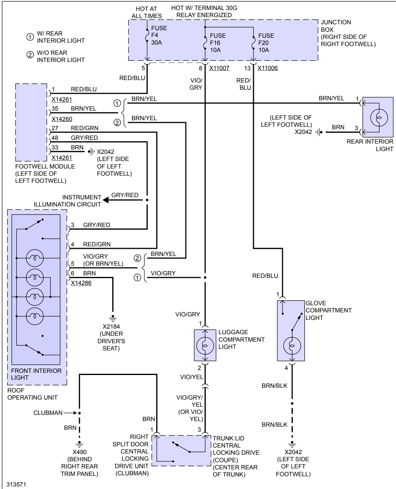
Fig 3: Courtesy Lamps Circuit, W/O Interior Lights Package
