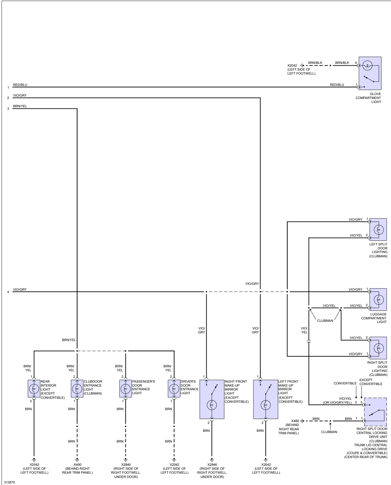
Fig 2: Courtesy Lamps Circuit, W/ Interior Lights Package (2 of 2)
