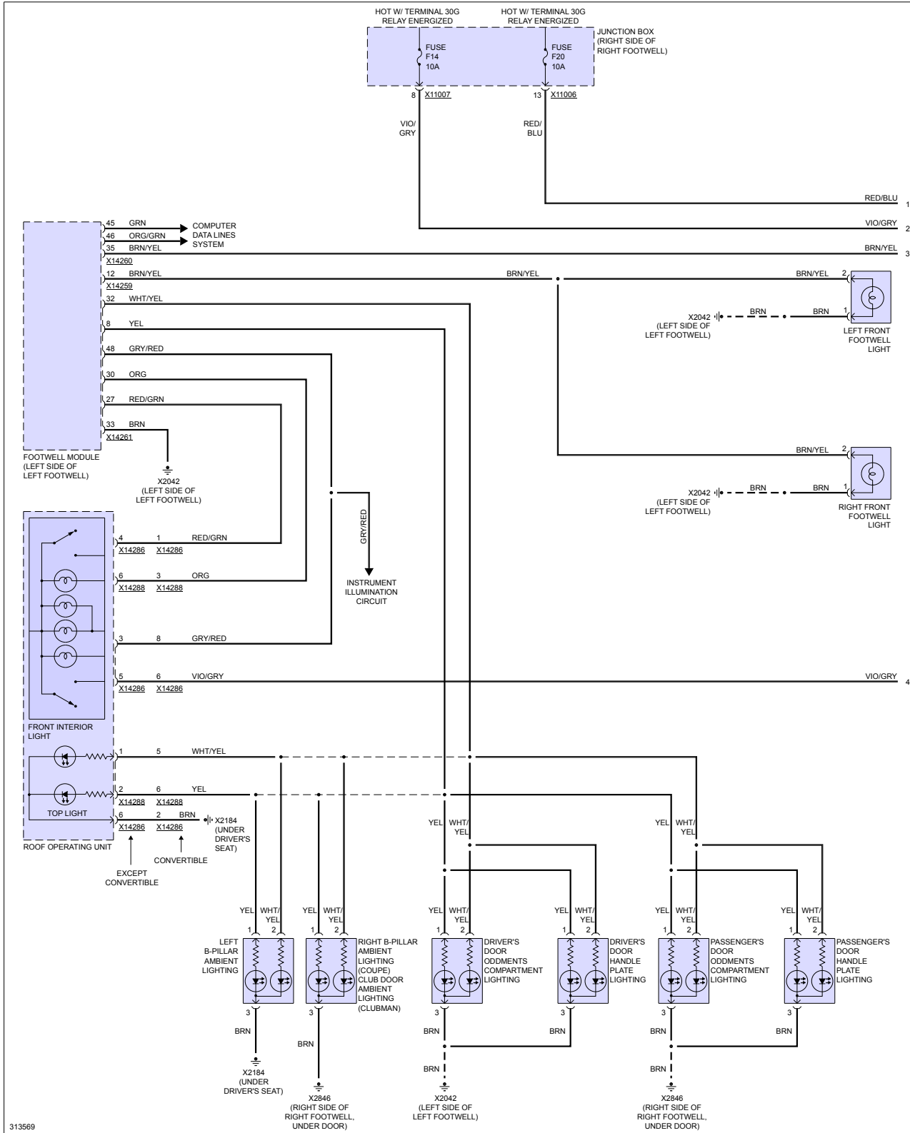
Fig 1: Courtesy Lamps Circuit, W/ Interior Lights Package (1 of 2)
