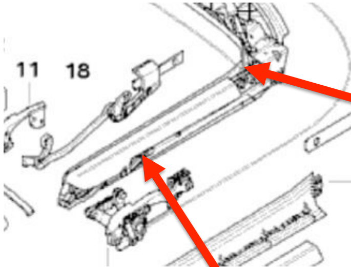
Front end of latching hook actuator rod
