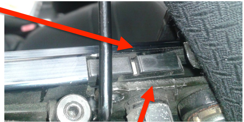
Aft end of latching hook actuator rod
