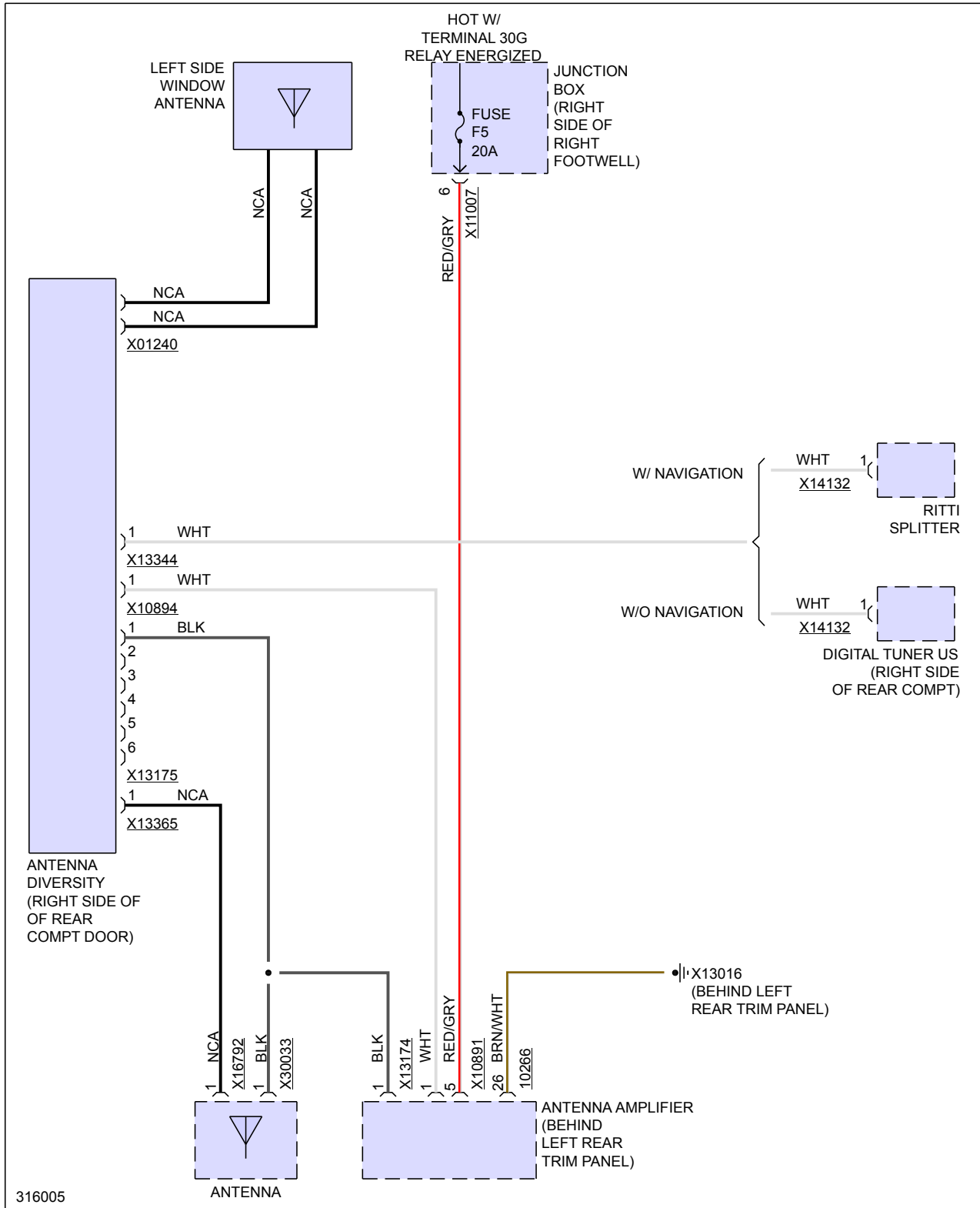
Fig 4: Diversity Antenna Circuit, Coupe W/ IBOC
